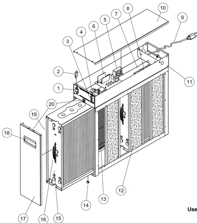
Fig. 7 — Exploded View
